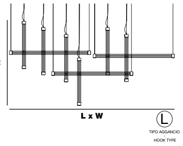
TRAMA S9 L x W 240 cm x 94 cm | 94,48" x 37" H 114 cm | 44,88" 9 - 360° neon flex 140,5W - 3000°K - 24 Vdc - SMD 2835T 16490,4 lm - life time 50.000 hrs - Dimmable: yes
