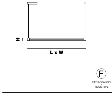
TRAMA S1 A L x W 126 cm x 6 cm | 49,61" x 2,36" H 6 cm | 2,36" 360° neon flex 21,6W - 3000°K - 24 Vdc - SMD 2835T 2536,8 lm - life time 50.000 hrs - Dimmable: yes
