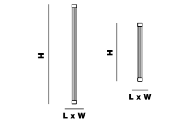
TRAMA WALL LAMP 120 - 70 L x W 6 cm x 8 cm | 2,36" x 3,15" H 126 cm | 49,61" / 75 cm | 29,53" 360° neon flex 21,6W/12,6W - 3000°K - 24 Vdc - SMD 2835T - 2536,8 lm/1480 lm - life time 50.000 hrs - Dimmable: yes
