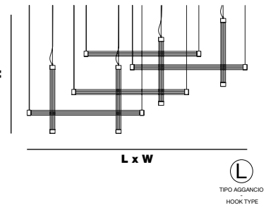
TRAMA S8 L x W 230 cm x 83 cm | 90,55" x 32,67" H 114 cm | 44,88" 8 - 360° neon flex 137W - 3000°K - 24 Vdc - SMD 2835T 16068 lm - life time 50.000 hrs - Dimmable: yes
