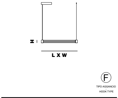
TRAMA S1 B L x W 75 cm x 6 cm | 29,53" x 2,36" H 6 cm | 2,36" 360° neon flex 12,6W - 3000°K - 24 Vdc - SMD 2835T 1480 lm - life time 50.000 hrs - Dimmable: yes
