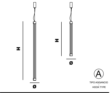
TRAMA S1 C - S1 D Ø 6 cm | 2,36" H 127 cm | 50" / 76 cm | 29,92" 360° neon flex 21,6W/12,6W - 3000°K - 24 Vdc - SMD 2835T - 2536,8 lm/1480 lm - life time 50.000 hrs - Dimmable: yes
