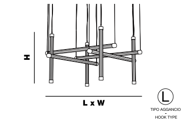
TRAMA S8 GRID L x W 126 cm x 126 cm | 49,61" x 49,61" H 76 cm | 29,92" 8 - 360° neon flex 137W - 3000°K - 24 Vdc - SMD 2835T 16068 lm - life time 50.000 hrs - Dimmable: yes
