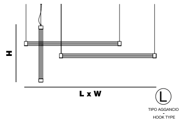
TRAMA S3 L x W 160 cm x 33 cm | 62,99" x 12,99" H 76 cm | 29,92" 3 - 360° neon flex 55,8W - 3000°K - 24 Vdc - SMD 2835T 6353,6 lm - life time 50.000 hrs - Dimmable: yes
