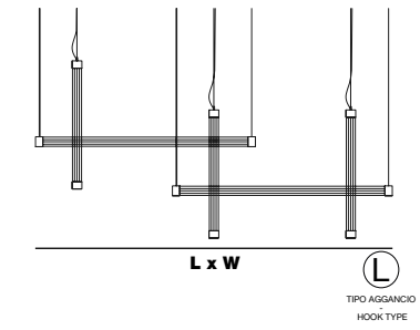
TRAMA S5 L x W 210 cm x 50 cm | 82,67" x 19,68" H 86 cm | 33,85" 5 - 360° neon flex 81W - 3000°K - 24 Vdc - SMD 2835T 9513,6 lm - life time 50.000 hrs - Dimmable: yes
